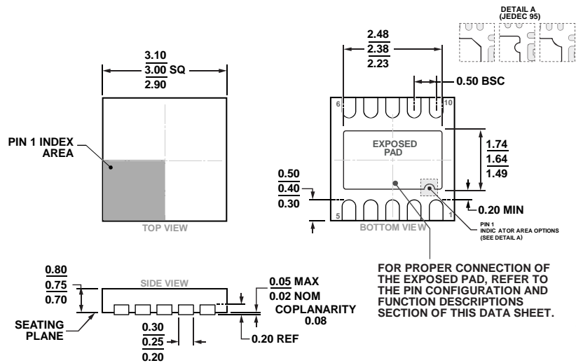
Figure 68. 10-Lead Lead Frame Chip Scale Package [LFCSP] 3 mm × 3 mm Body and 0.75 mm Package Height (CP-10-9) Dimensions shown in millimeters
