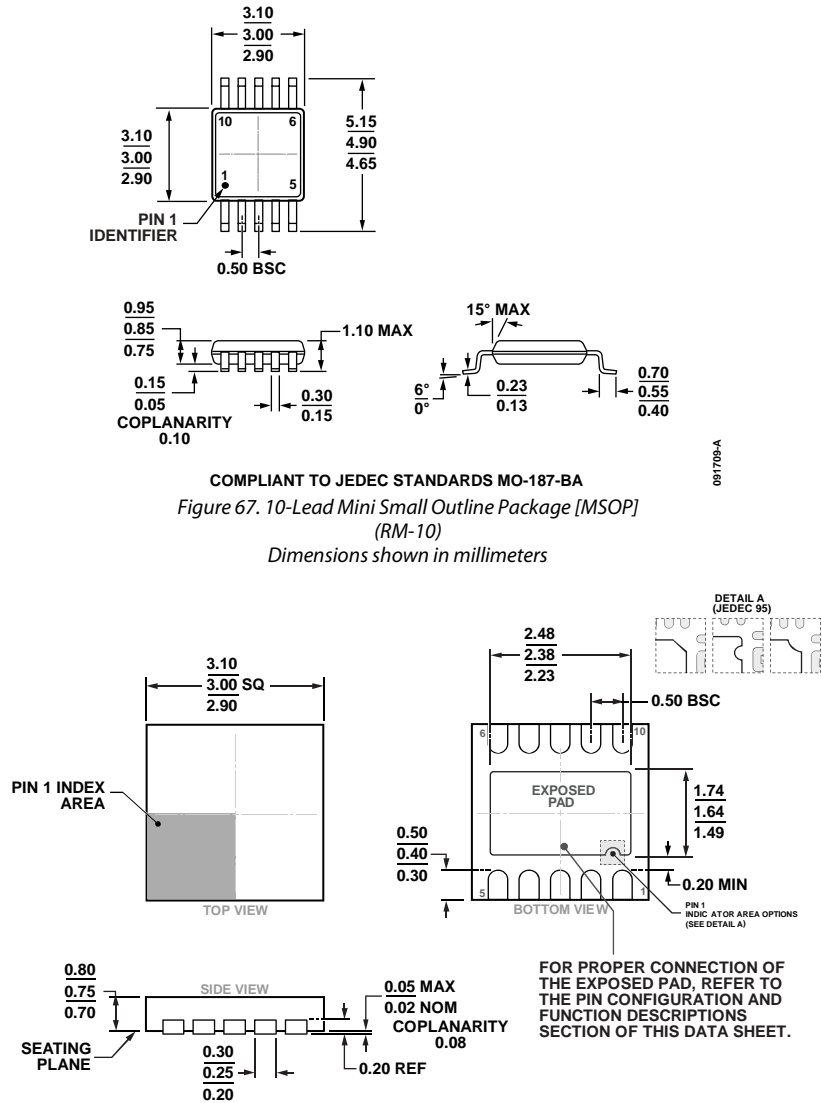
Figure 68. 10-Lead Lead Frame Chip Scale Package [LFCSP] 3 mm × 3 mm Body and 0.75 mm Package Height (CP-10-9) Dimensions shown in millimeters
