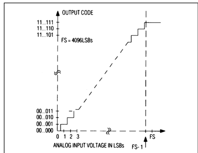
Figure 17. MX7672 Ideal Unipolar Transfer Function
