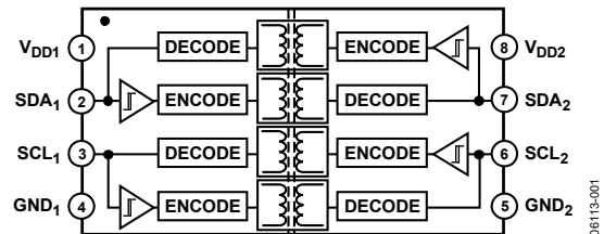
Figure 1. ADuM1250
