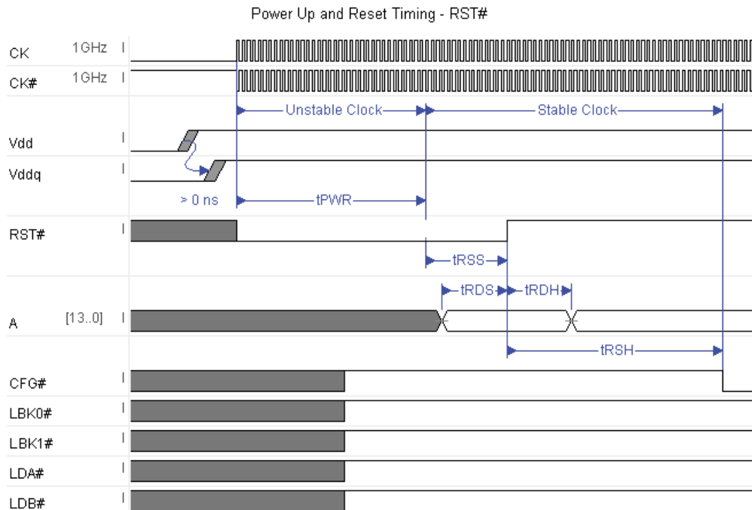
Figure 16. Reset Timings
