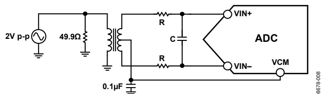
Figure 38. Differential Transformer-Coupled Configuration
