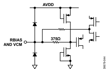
Figure 34. Equivalent RBIAS and VCM Circuit
