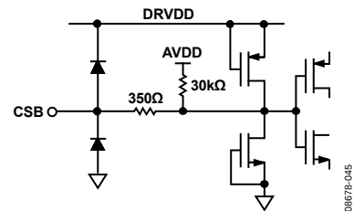
Figure 33. Equivalent CSB Input Circuit
