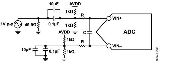
Figure 39. Single-Ended Input Configuration
