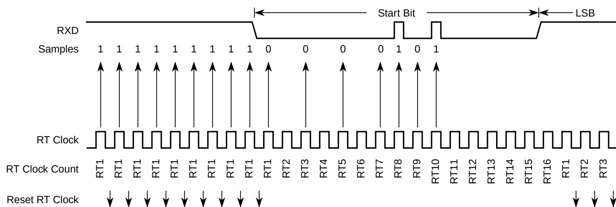
In Figure 14-27 , a noise burst makes the majority of data samples RT8, RT9, and RT10 high. This sets the noise flag but does not reset the RT clock. In start bits only, the RT8, RT9, and RT10 data samples are ignored.
