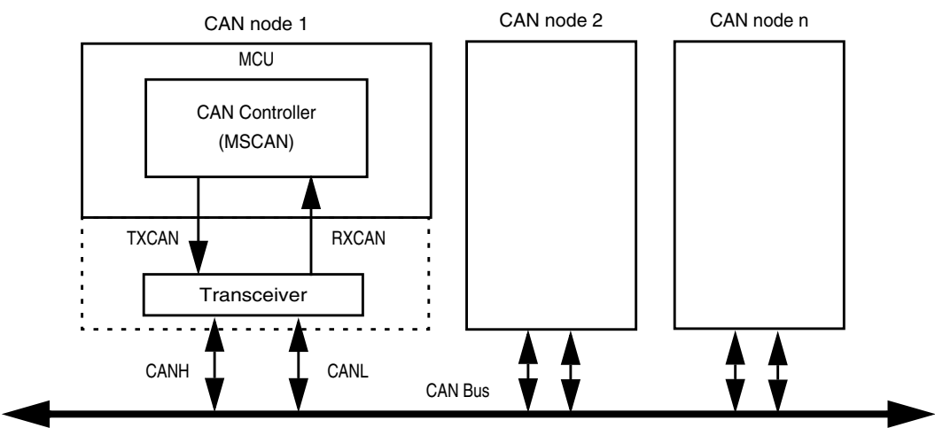
Figure 11-2. CAN System
