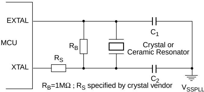
Figure 1-7. Full Swing Pierce Oscillator Connections (XCLKS = 1)
