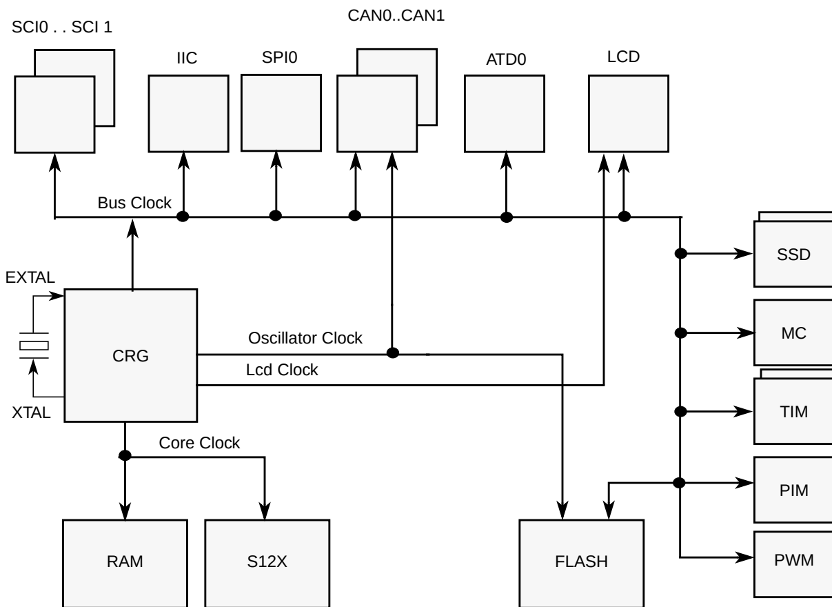
Figure 1-5. Clock Connections
