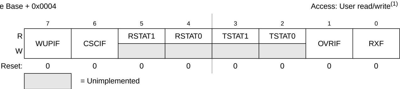
Figure 11-8. MSCAN Receiver Flag Register (CANRFLG)
