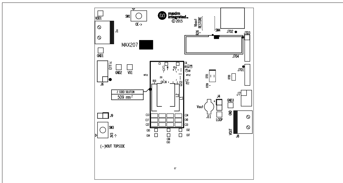
Top Silkscreen
