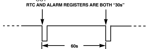
FIGURE 14. \overline{\text{IRQ}}/\text{F}_{\text{OUT}} WAVEFORM
