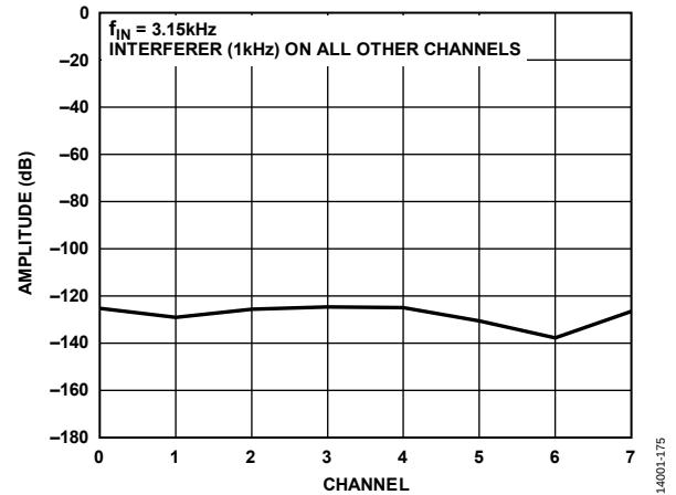
Figure 33. Crosstalk
