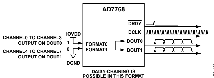
Figure 96. AD7768 FORMAT x = 01, Two Data Output Pins
