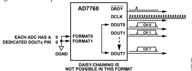
Figure 95. AD7768 FORMAT x = 00, Eight Data Output Pins
