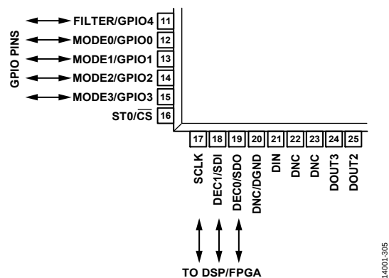
Figure 114. AD7768-4 GPIO Functionality
