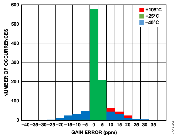
Figure 51. Gain Error Distribution
