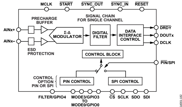
Figure 83. Top Level Core Signal Chain and Control
