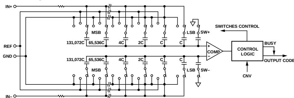
Figure 21. ADC Simplified Schematic
