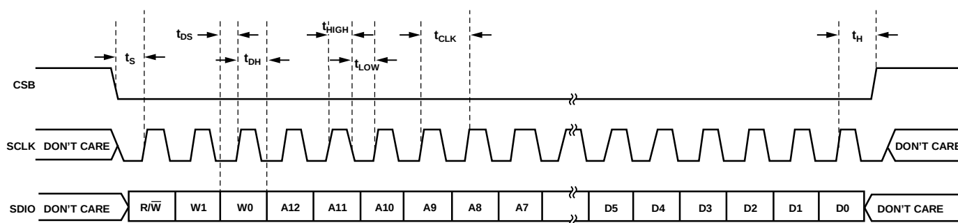
Figure 55. Serial Port Interface Timing Diagram
