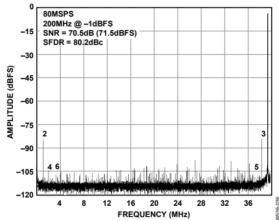
Figure 8. AD9649-80 Single-Tone FFT with f_{IN} = 200 MHz
