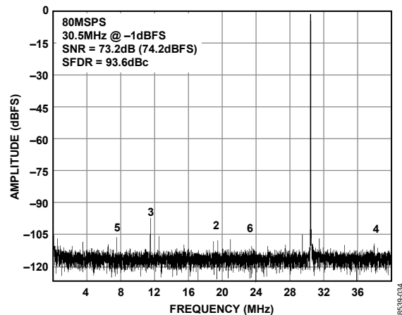
Figure 7. AD9649-80 Single-Tone FFT with f_{IN} = 30.5 MHz
