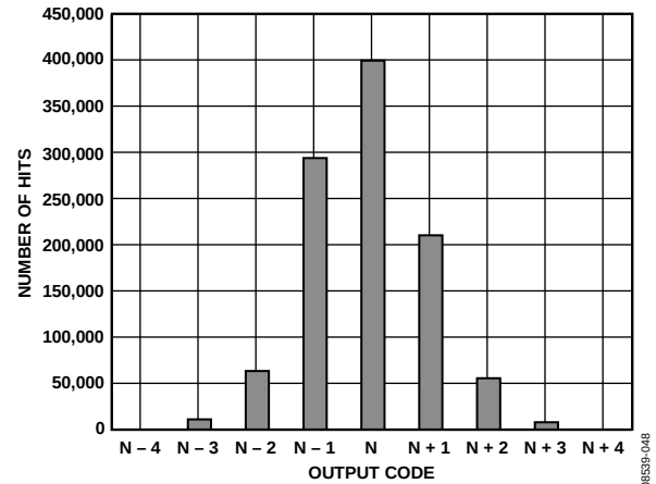
Figure 14. AD9649-80 Grounded Input Histogram
