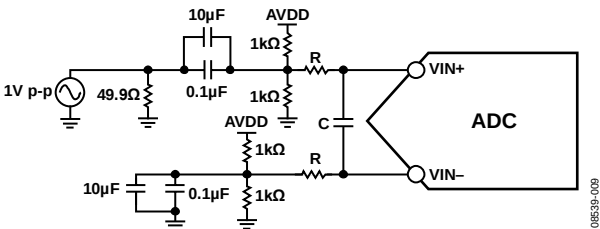
Figure 40. Single-Ended Input Configuration
