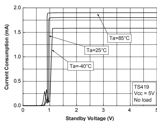
Figure 15. Current consumption vs. standby voltage Vcc = 5 V
