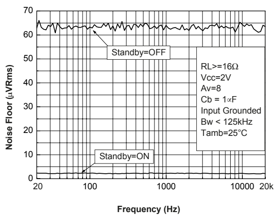
Figure 92. Noise floor Vcc = 2 V
