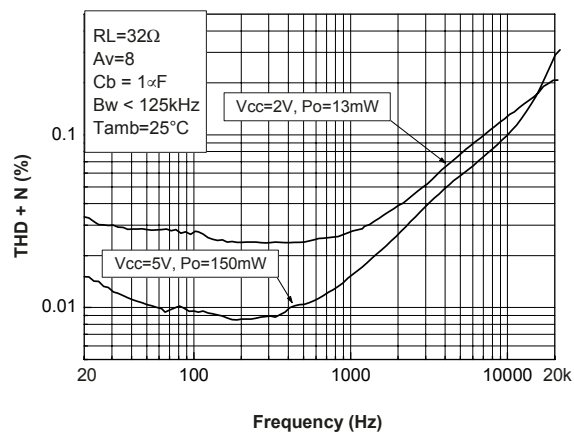
Figure 88. THD + N vs. frequency R_L = 32\ \Omega
