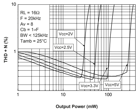
Figure 84. THD + N vs. output power R_L = 16\ \Omega , C_b = 1\ \mu\text{F}
