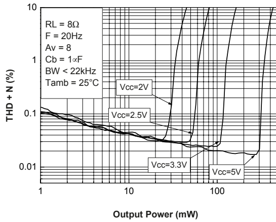
Figure 77. THD + N vs. output power R_L = 8\ \Omega
