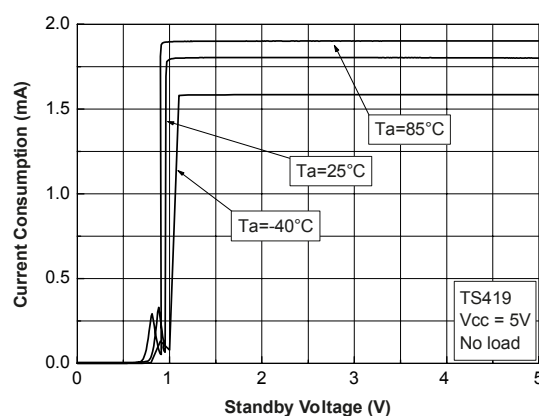
Figure 15. Current consumption vs. standby voltage V_{CC} = 5\text{ V}
