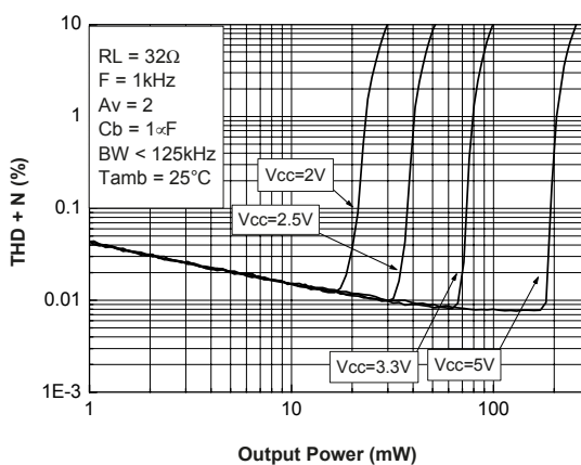
Figure 40. THD + N vs. output power R_L = 32\ \Omega , A_v = 2
