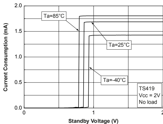
Figure 17. Current consumption vs. standby voltage V_{CC} = 2\text{ V}
