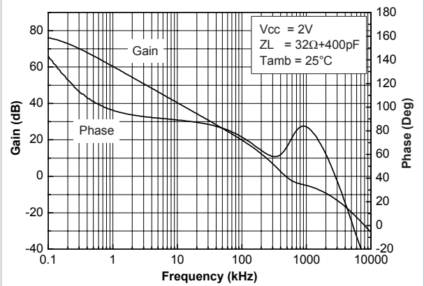
Figure 13. Open loop gain and phase vs. frequency ZL = 32 \Omega , V_{CC} = 2V
