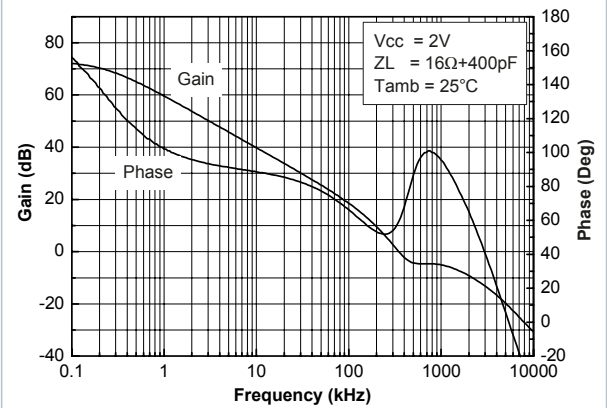
Figure 9. Open loop gain and phase vs. frequency ZL = 16 \Omega , Vcc = 2 V
