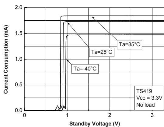
Figure 16. Current consumption vs. standby voltage V_{CC} = 3.3\text{ V}
