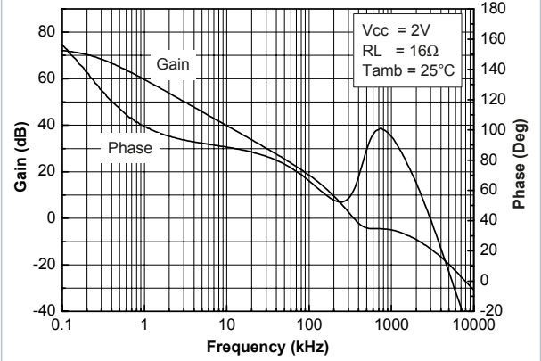
Figure 7. Open loop gain and phase vs. frequency RL = 16 \Omega , Vcc = 2 V
