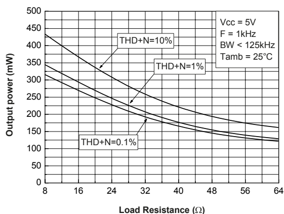
Figure 25. Output power vs. load resistor Vcc = 5 V
