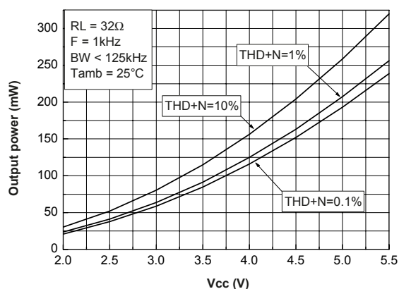
Figure 23. Output power vs. power supply voltage RL = 32 \Omega
