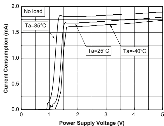
Figure 14. Current consumption vs. power supply voltage
