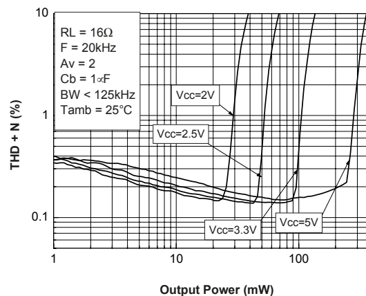
Figure 42. THD + N vs. output power R_L = 16\ \Omega , C_b = 1\ \mu F
