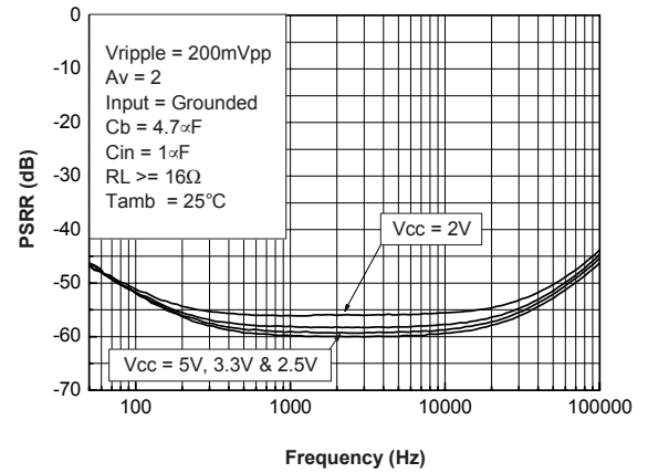
Figure 54. PSRR vs. bypass capacitor C_b = 4.7\ \mu\text{F}
