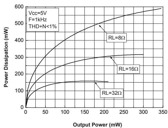
Figure 29. Power dissipation vs. output power V CC = 5 V
