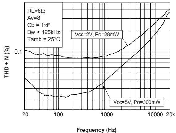
Figure 86. THD + N vs. frequency R_L = 8\ \Omega
