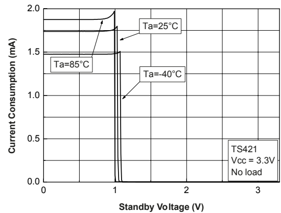
Figure 19. Current consumption vs. standby voltage V_{CC} = 3.3\text{ V} (TS421)
