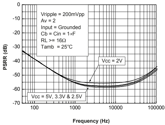
Figure 53. PSRR vs. bypass capacitor C_b = C_{in} = 1\ \mu\text{F}
