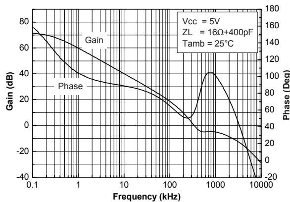
Figure 8. Open loop gain and phase vs. frequency ZL = 16 \Omega , Vcc = 5 V
