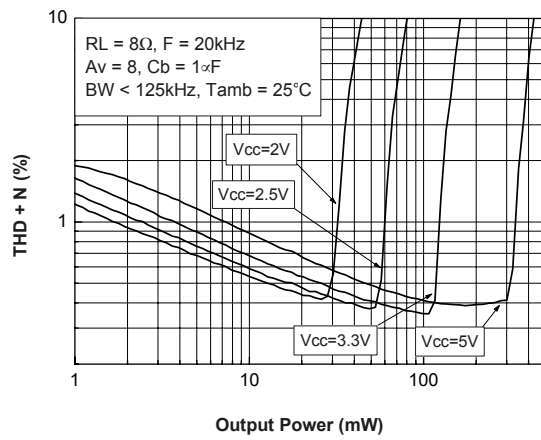
Figure 83. THD + N vs. output power R_L = 8\ \Omega , C_b = 1\ \mu\text{F}
