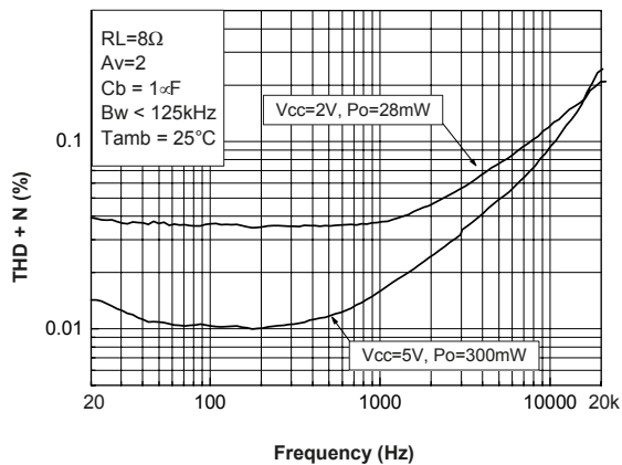
Figure 44. THD + N vs. frequency R_L = 8\ \Omega
