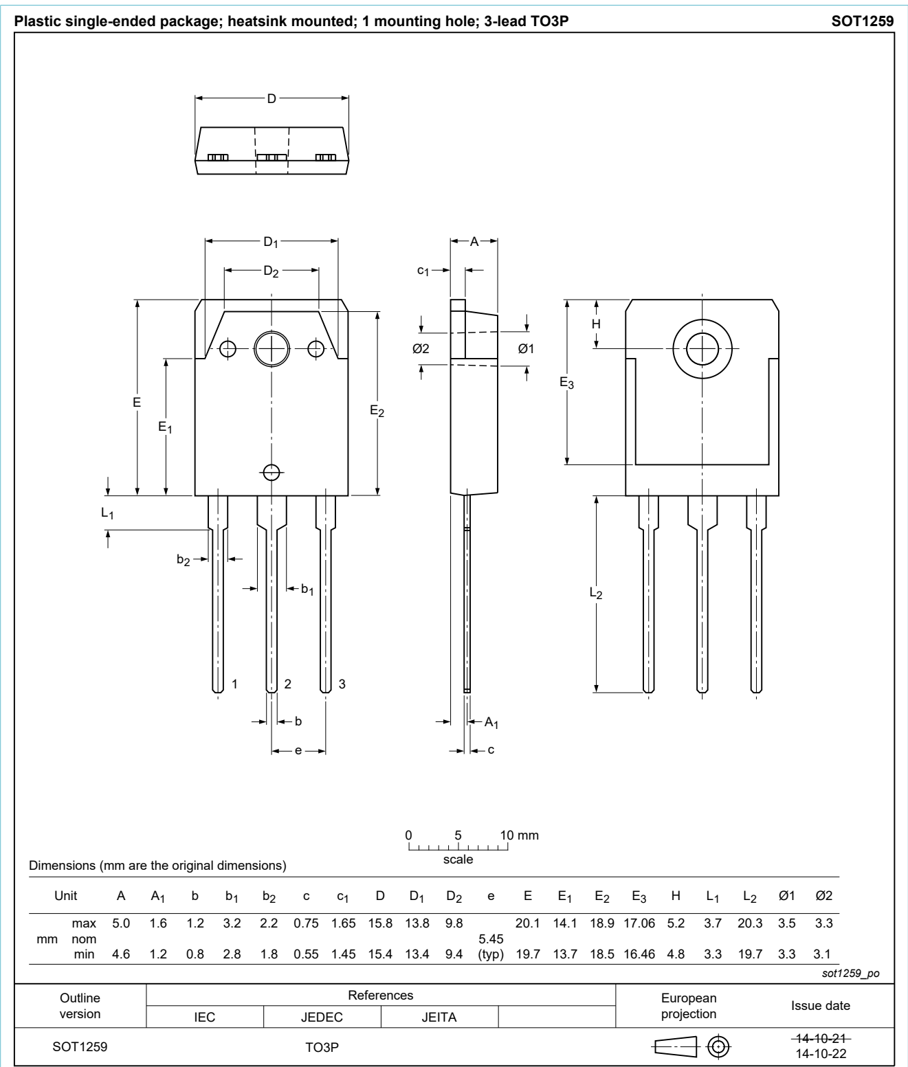
Fig. 13. Package outline TO3P (SOT1259)
