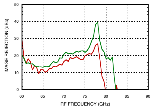
Image Rejection, LSB vs. LO Drive
