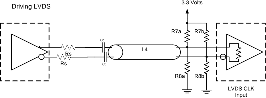
Driving LVDS inputs
