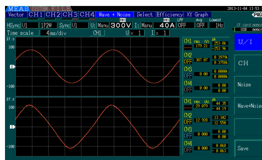
Figure 20. 100% Load
