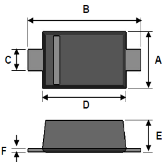
SOD-123F
