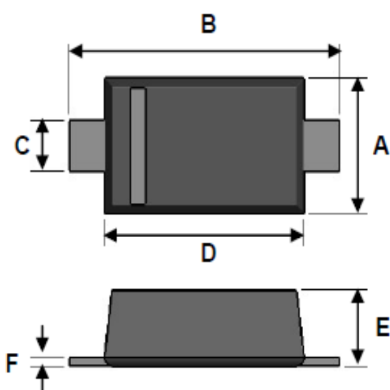
SOD-123F
