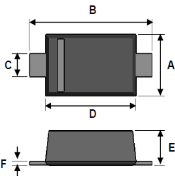
SOD-123F
