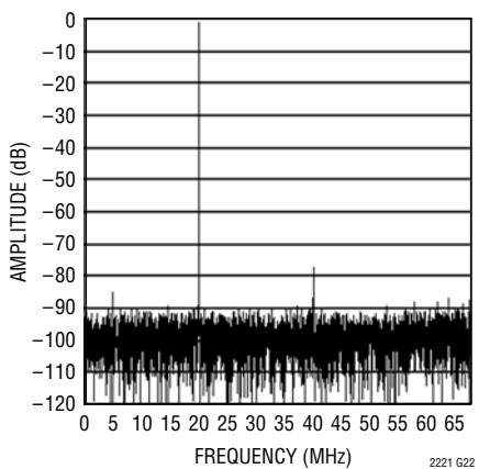
LTC2221: 8192 Point FFT, f_{IN} = 250\text{MHz} , -1\text{dB} , 1\text{V} Range, LVDS Mode
