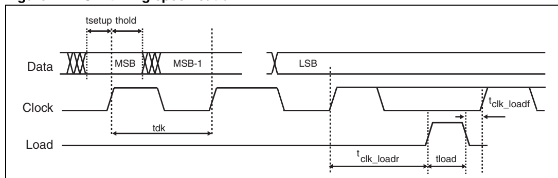
Figure 27. SPI timing specification
