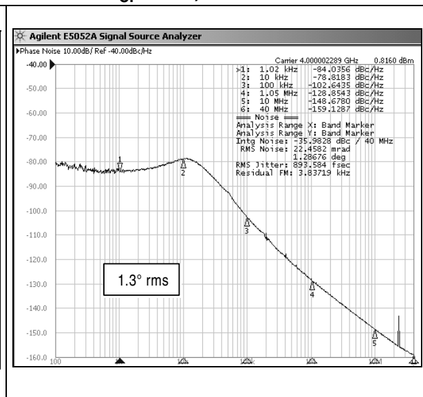
Figure 6. VCO B (direct output) closed loop phase noise at 4.0 GHz ( F_{\text{STEP}}=200 kHz; F_{\text{PFD}}=200 kHz; I_{\text{CP}}=4 mA)
