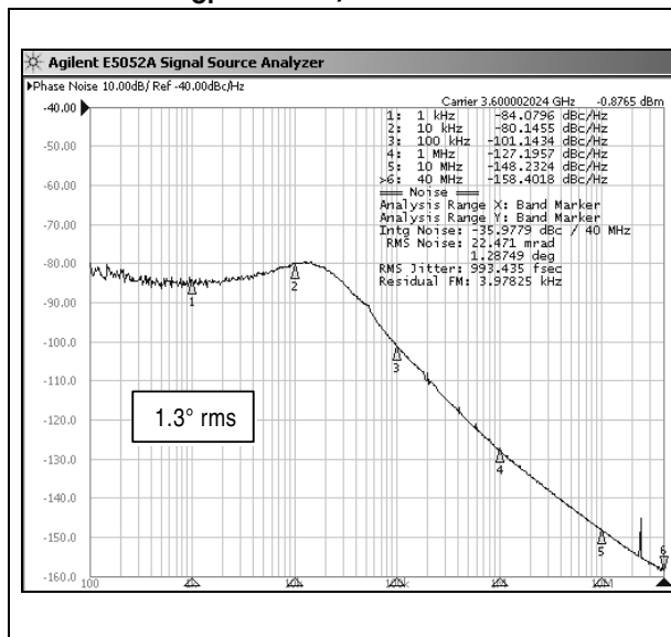
Figure 5. VCO A (direct output) closed loop phase noise at 3.6 GHz ( F_{\text{STEP}}=200 kHz; F_{\text{PFD}}=200 kHz; I_{\text{CP}}=3.5 mA)
