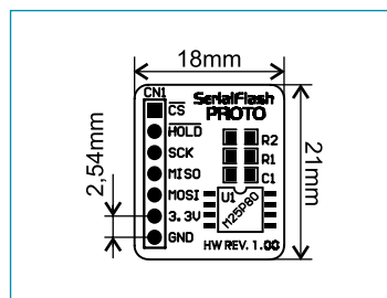
Figure 4: Dimensions of the board
