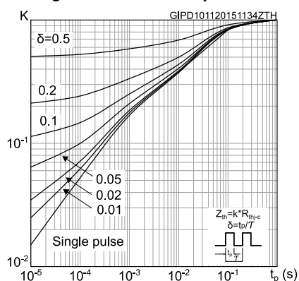
Figure 3: Thermal impedance
