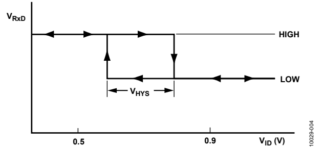
Figure 26. Receiver Input Hysteresis
