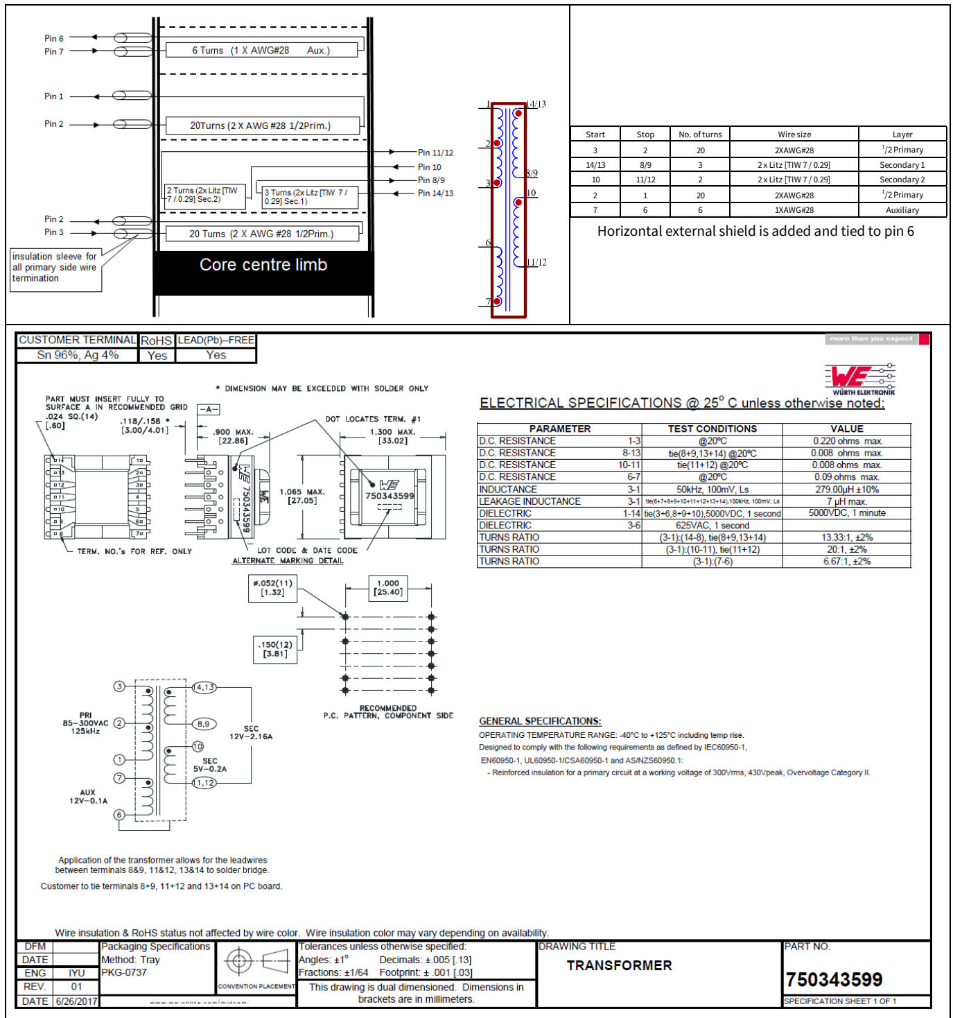
Figure 7 Transformer structure
