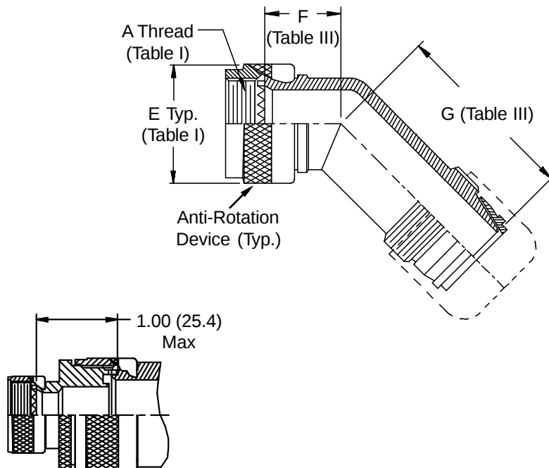
STYLE 2 (See Note 1)
