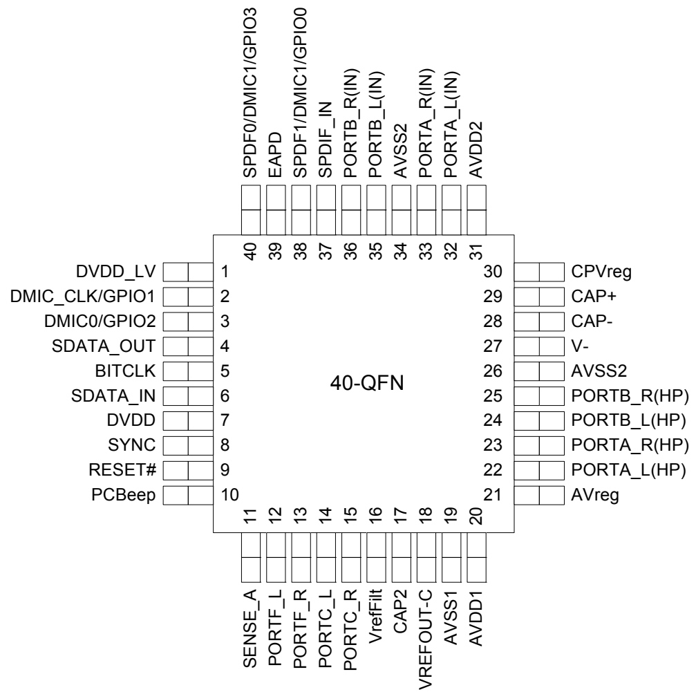
Figure 15. 40-Pin Pinout
