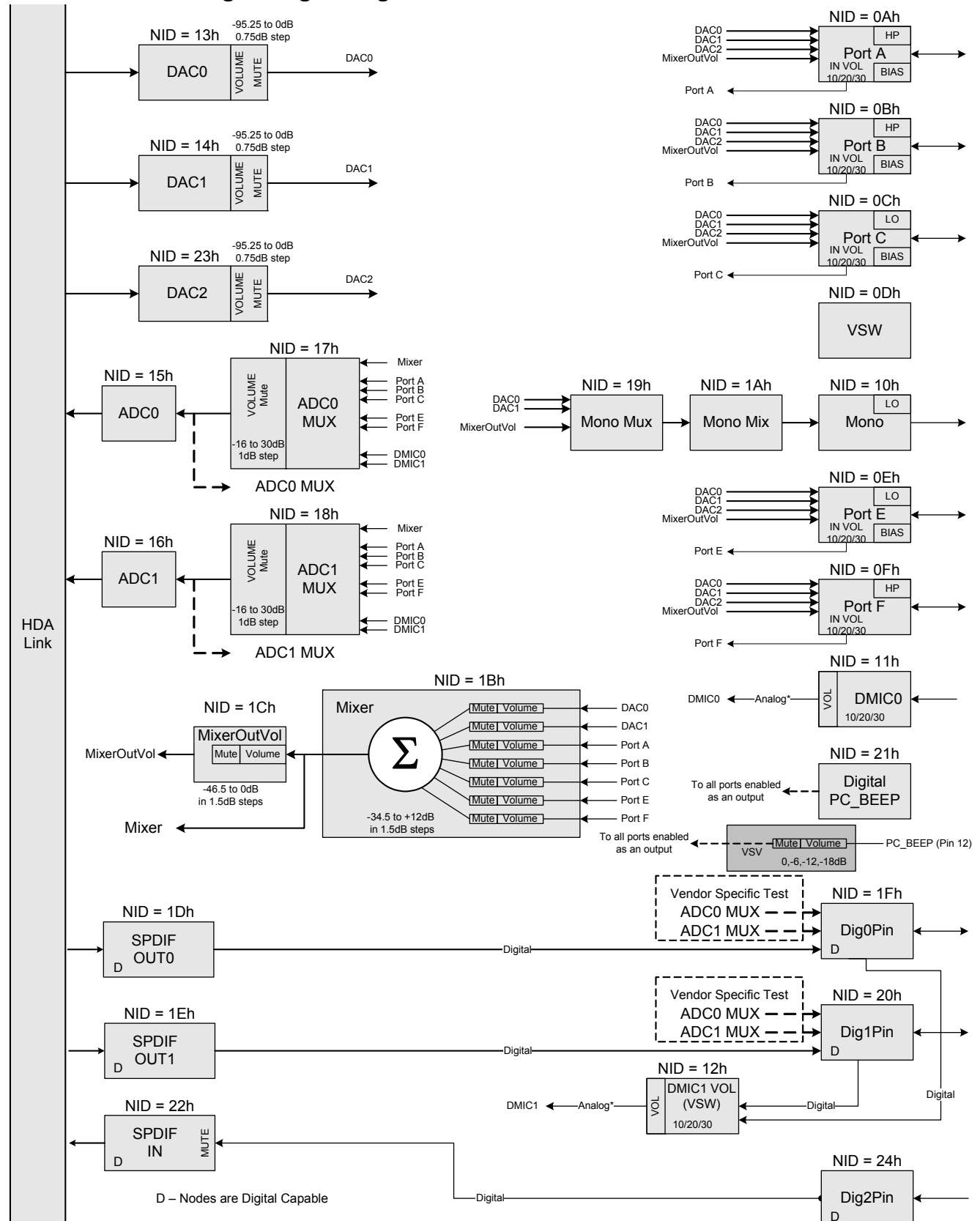
Figure 12. 48-pin Package Widget Diagram
