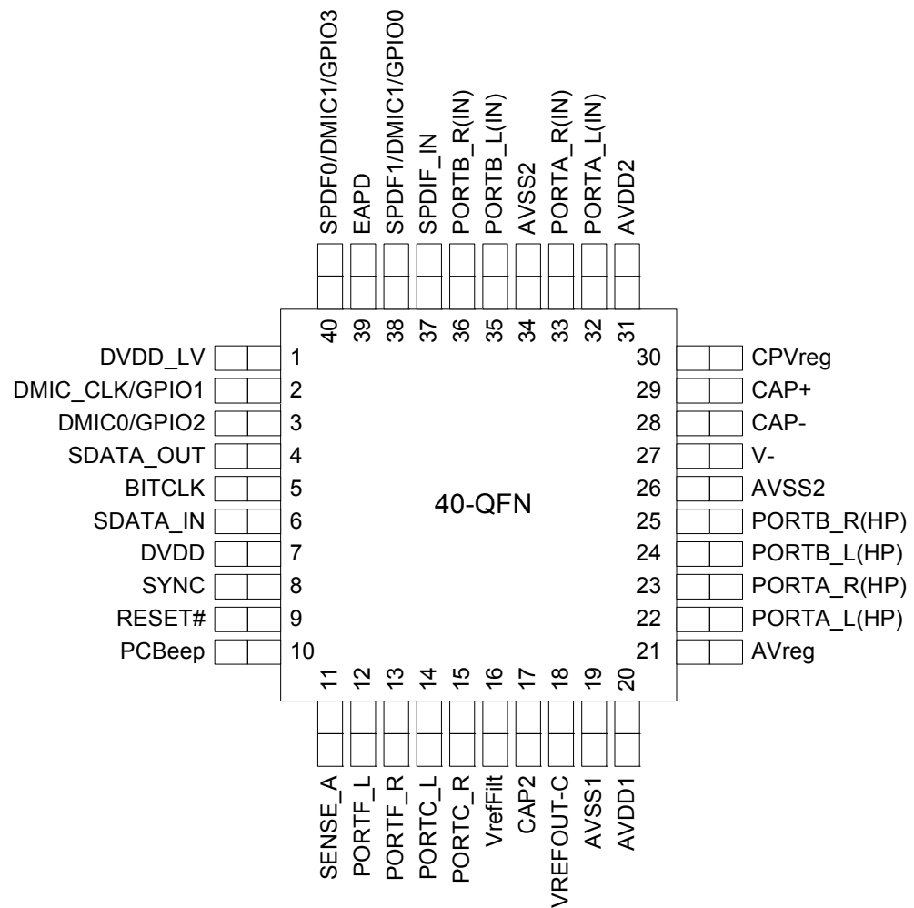
Figure 15. 40-Pin Pinout
