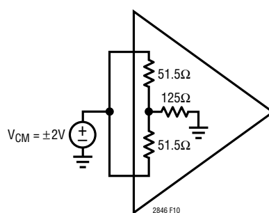
Figure 10. Receiver Common Mode Impedance Test Circuit
