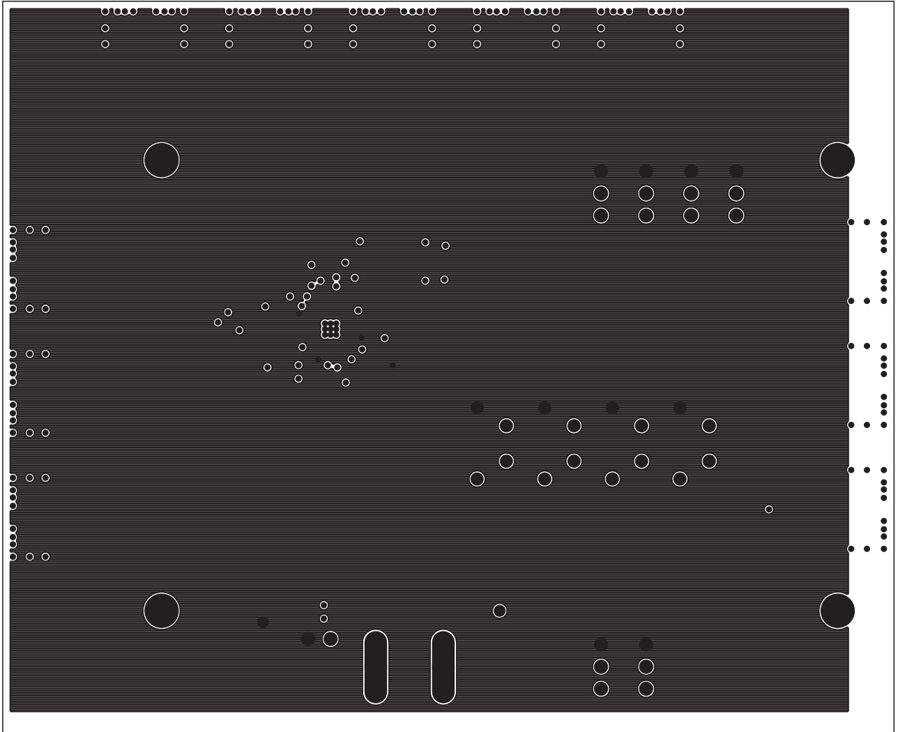
Figure 5. MAX3679A EV Kit Layout—Power Plane
