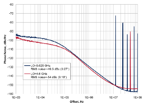
Figure 14. Phase noise at 5.625 GHz and 4.6 GHz ( F_{\text{PFD}} = 50 \text{ MHz} )
