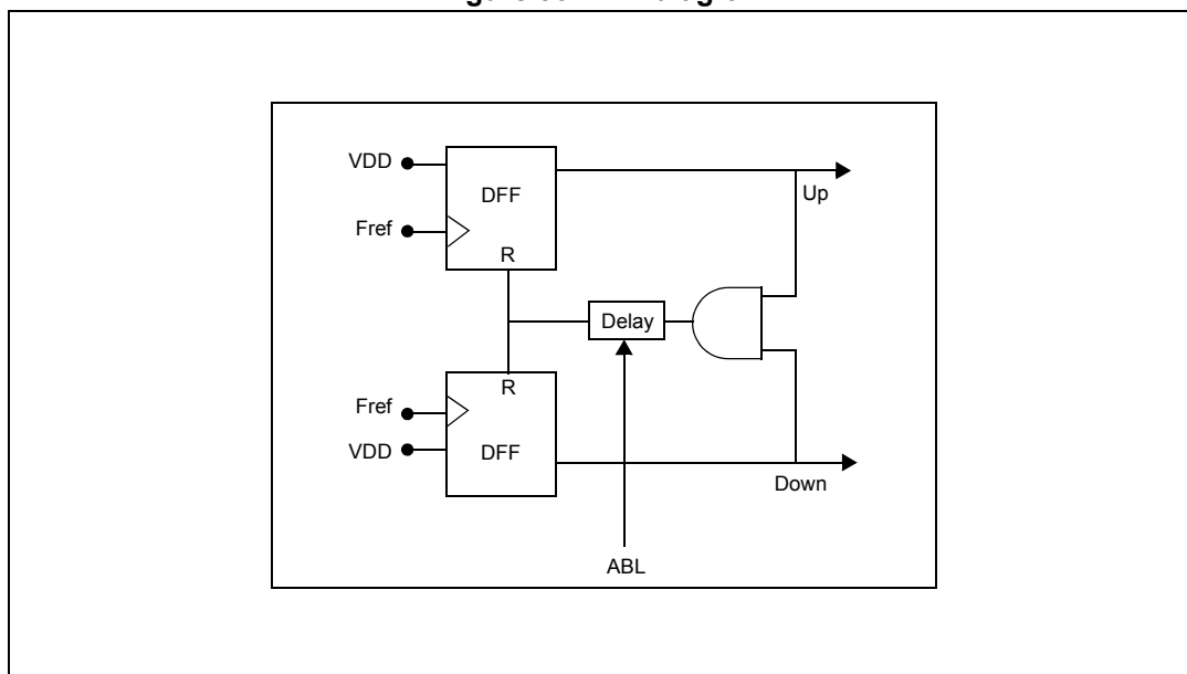
Figure 30. PFD diagram
