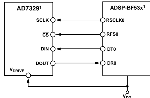
Figure 59. Interfacing the AD7329 to the ADSP-BF53x
