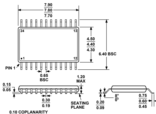
Figure 61. 24-Lead Thin Shrink Small Outline Package [TSSOP] (RU-24) Dimensions shown in millimeters
