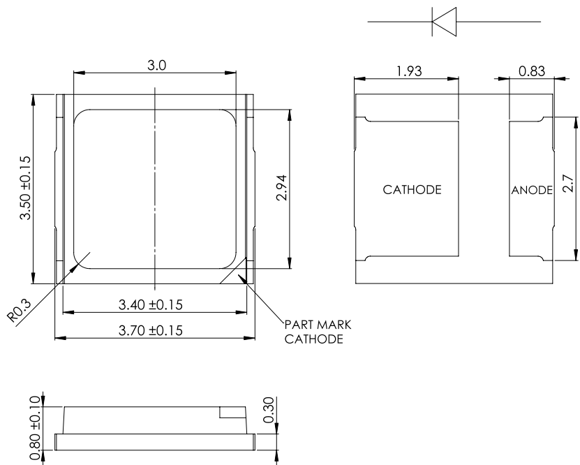
Figure 9b. Mechanical dimensions for L135-xxxxSA35000P1.
