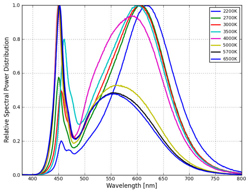
Figure 1b. Typical normalized power vs. wavelength for 80CRI LUXEON 3535L Line at 100mA, T j =25°C.
