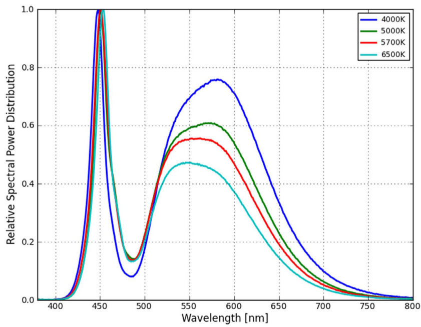
Figure 1a. Typical normalized power vs. wavelength for 70CRI LUXEON 3535L Line at 100mA, T j =25°C.
