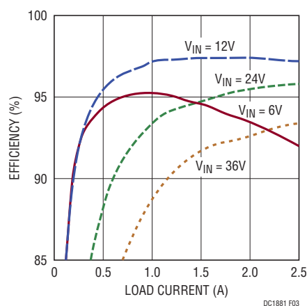
Figure 3. Efficiency vs Load Current ( V_O = 12V , CCM)
