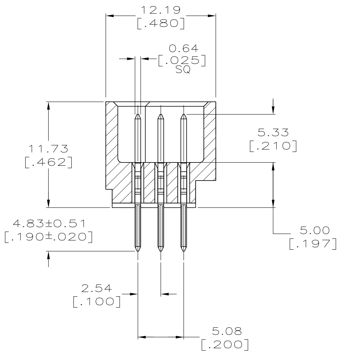
SECTION T-T
