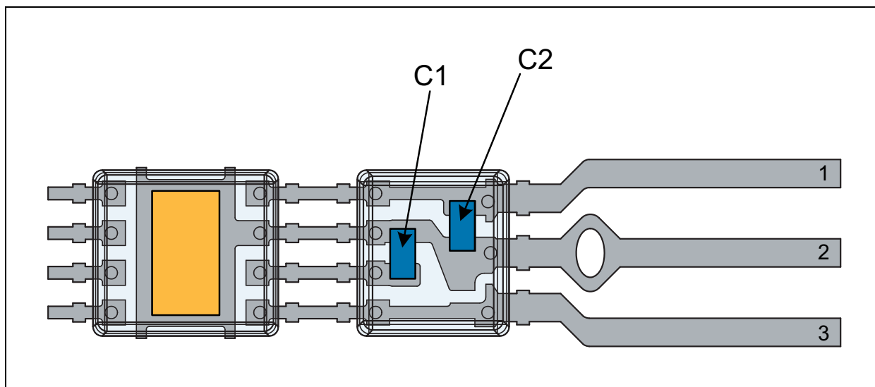
Figure 74: AS5172A Components
