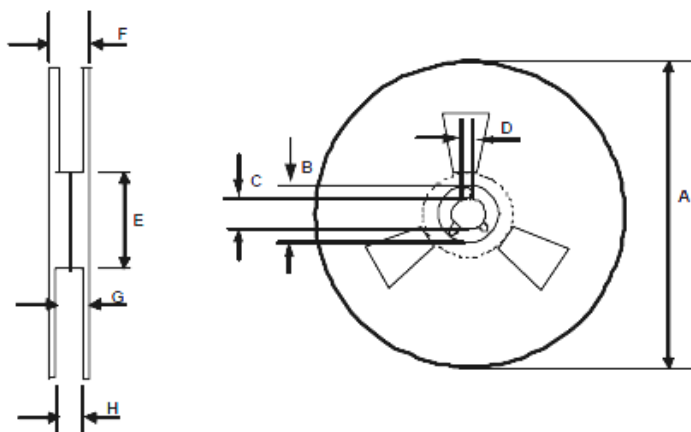
REEL DIMENSIONS FOR 14SO14N
