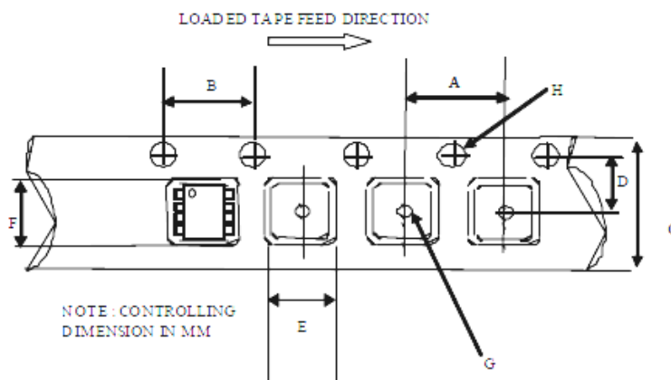
CARRIER TAPE DIMENSION FOR 14SO14N
