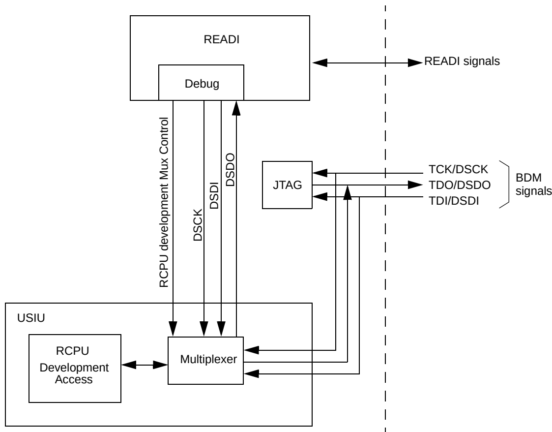
Figure 23-77. RCPU Development Access Multiplexing between READI and BDM Signals
