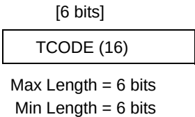
Figure 23-54. Target Ready Message
