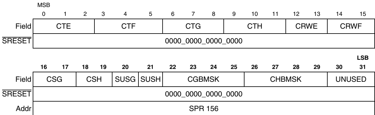
Figure 22-21. L-Bus Support Control Register 1 (LCTRL)
