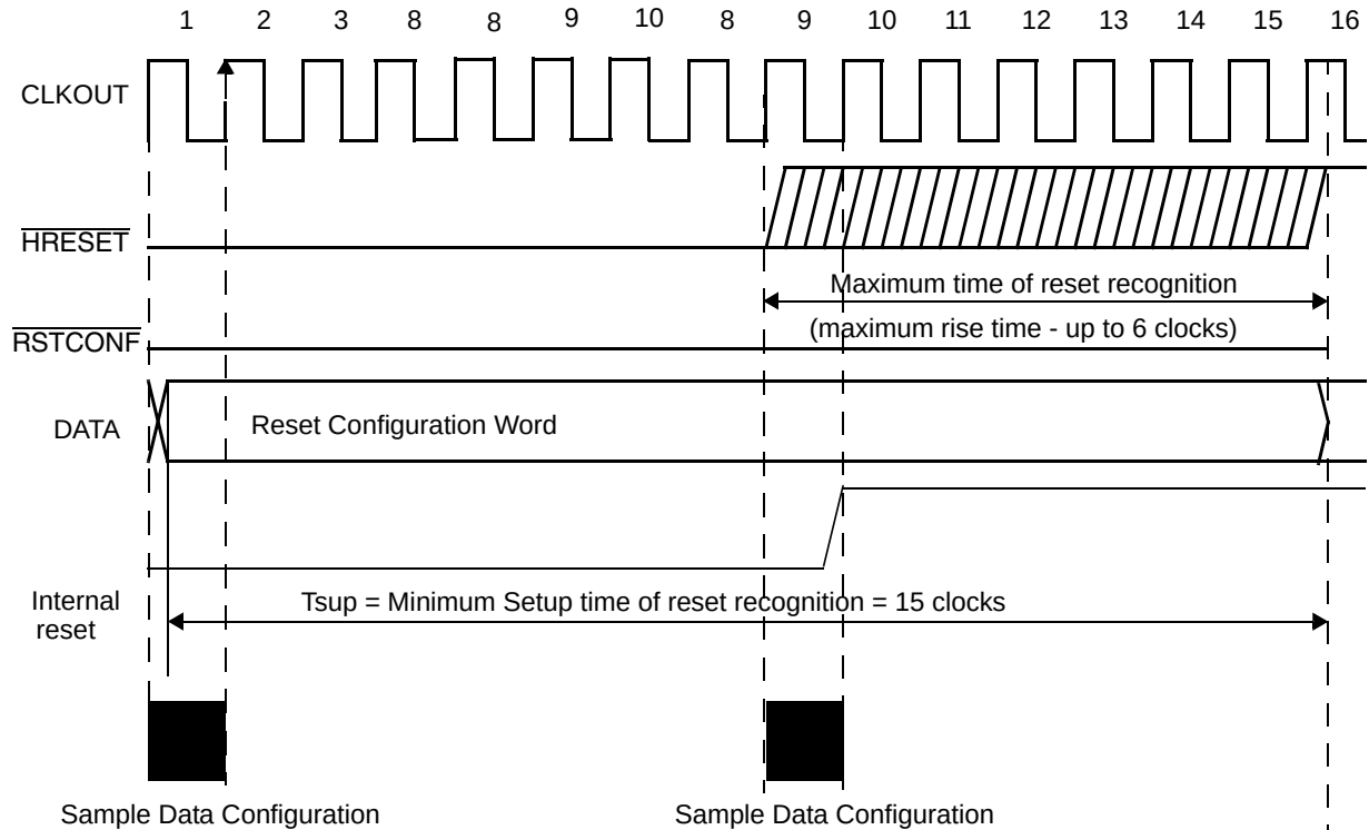
Figure 7-6. Reset Configuration Sampling Timing Requirements
